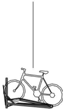
Haniss Single Height - Three Spots H=855, W=1220, D=1563.7
